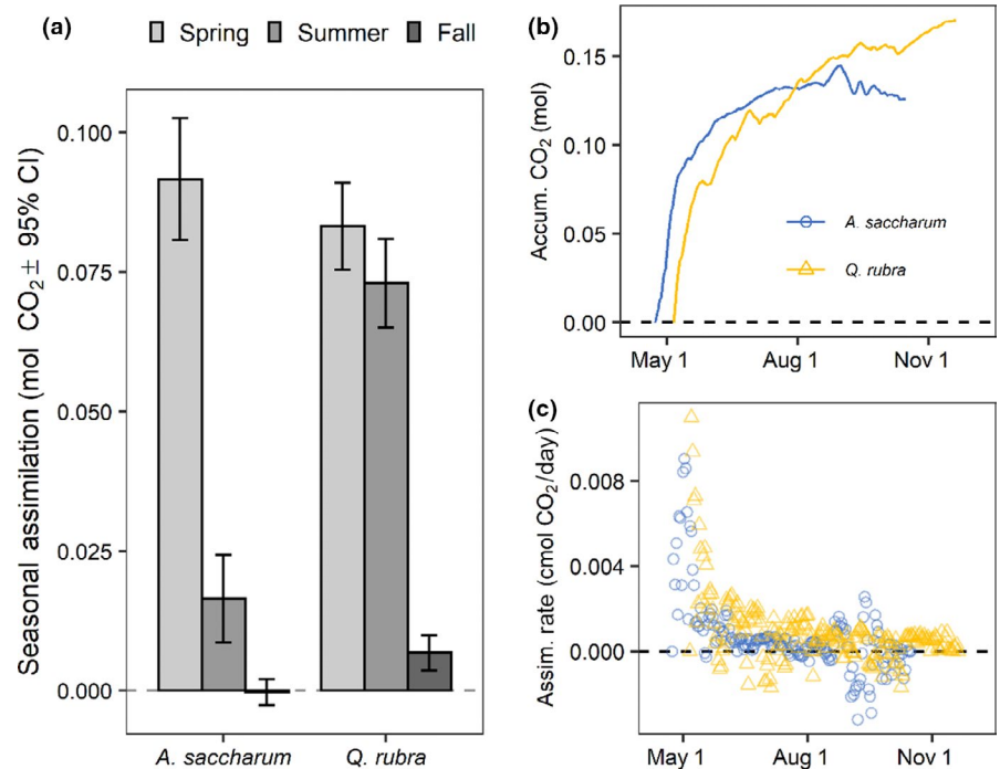
FIGURE 1 (a) Average tree seedling net foliar CO 2 assimilation estimates ( \pm 95\% confidence intervals) for spring, summer and fall. Panels on the right show examples of (b) additive CO 2 assimilation and (c) average daily assimilation rates for representative Acer saccharum (blue, circles) and Quercus rubra (yellow, triangles) individuals
